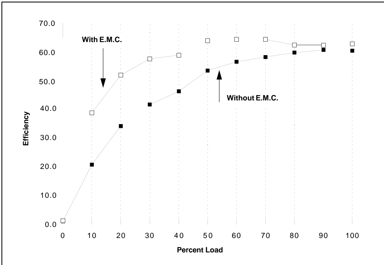
FIGURE 4: MOTOR EFFICIENCY
